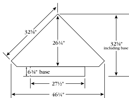
Corner Mantel (36 1/2" high)
