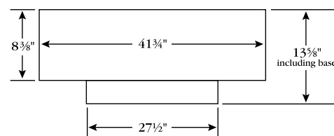
Cabinet Mantel (36 1/2" high)
